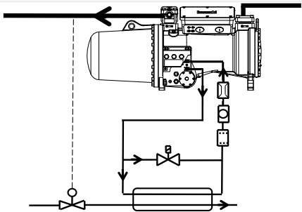
Typical circuit
